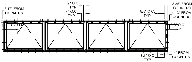
TYPICAL ELEVATION WITH FASTENER SPACING
