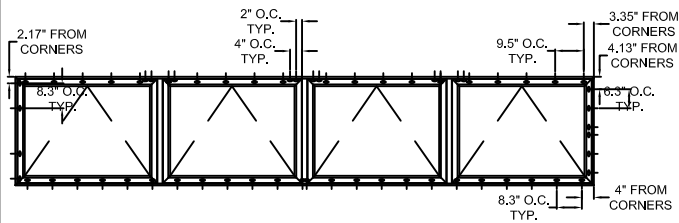
TYPICAL ELEVATION WITH FASTENER SPACING
