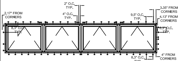
TYPICAL ELEVATION WITH FASTENER SPACING
