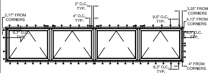
TYPICAL ELEVATION WITH FASTENER SPACING
